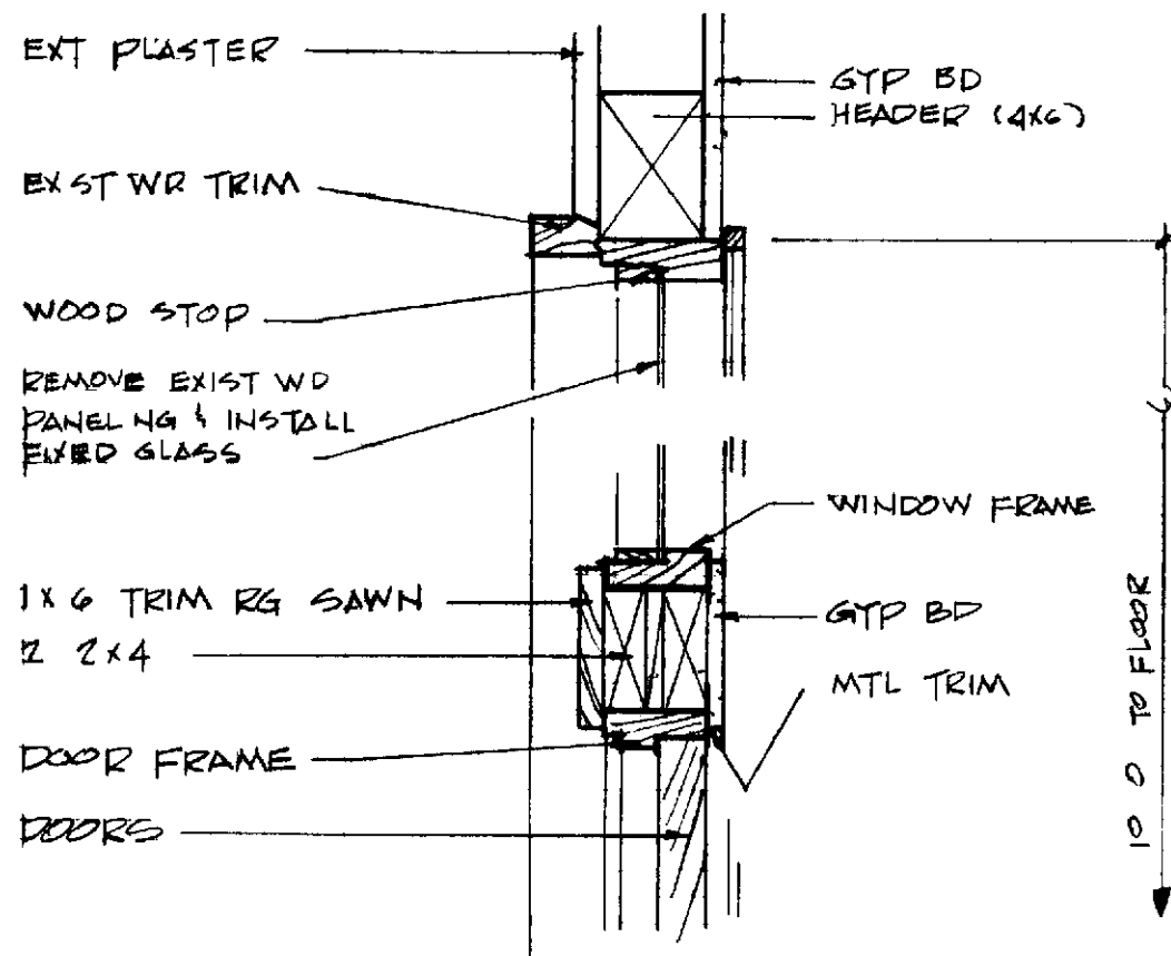
SECTION OF WINDOW SCALE 1 1/2" = 1' 0"
