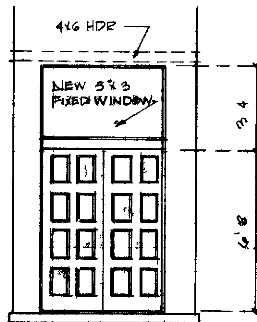
ELEVATION OF FRONT DOOR SCALE 1/4" = 0'
